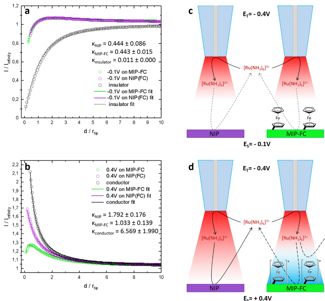
Fig. 7 SECM studies performed in feedback mode. Approach curves recorded on post-imprinting modified and non-imprinted macroporous film samples biased at (a) -0.1\text{ V} and (b) 0.4\text{ V} vs. \text{Ag}_{\text{pseudo}} . Schemes showing post-imprinted and non-imprinted macroporous film behavior at (c) -0.1\text{ V} and (d) +0.4\text{ V} biased potential. E_S -potential applied to the sample electrode, E_T -potential applied over Pt microelectrode tip.
