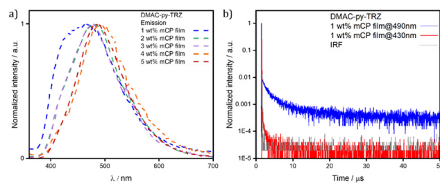
Fig. 7 (a) Emission spectra of DMAC-py-TRZ in spin-coated 1–5 wt% mCP films ( \lambda_{exc} = 340 nm); (b) time-resolved PL decay in spin-coated 1 wt% mCP film of DMAC-py-TRZ collected at \lambda_{em} = 490 nm and \lambda_{em} = 430 nm ( \lambda_{exc} = 378 nm).
