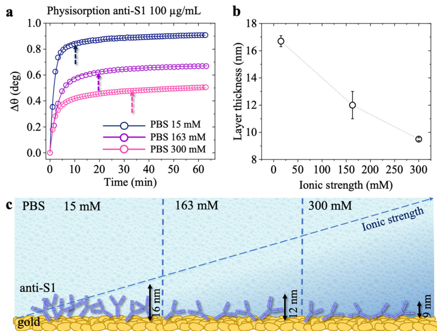
Fig. 3 (a) SPR sensograms ( \Delta\theta vs. time) of the physorption of anti-S1 on the SPR gold slide in PBS buffer at different ionic strengths. The hollow circles refer to physorption in PBS solution at i_s 15 mM (blue), 163 mM (purple) and 300 mM (magenta). The pH in all cases is kept constant at 7.4. The full lines are the fittings of the traces measured at the different ionic strengths. The dashed arrow indicates the minimum time required for the physorption to reach 95% surface coverage. (b) Average values of the simulated thickness values. Error bars are the relative standard deviation of simulations performed on two different sampled areas. (c) Schematic illustration of anti-S1 physorption onto the gold SPR slide at different ionic strengths.
