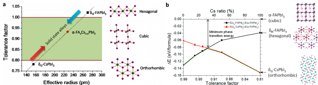
Fig. 2 (a) Correlations between the tolerance factor and crystal structure of perovskite materials. (b) Calculated energy difference between the \alpha -phase and different \delta -phases for FA 1-x Cs x PbI 3 alloys with different Cs ratios. Adapted with permission from ref. 55.
