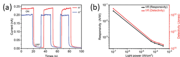
Fig. 36 (a) Photocurrent during L- and R-CPL irradiation at 430 nm and (b) responsivity and detectivity vs. power intensity at 430 nm of ( R -3AMP)PbBr _4 . Reprinted with permission from ref. 41 Copyright©2022 Wiley-VCH GmbH.
