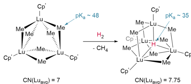
Fig. 4 Despite the higher pK a of the methyl anion hydrogenolysis occurs with Hou's trimer due to the coordinative stabilisation provided by the μ 4 -hydride in the tetrameric product. CN = coordination number; Cp' = (C 5 H 4 SiMe 3 )†
