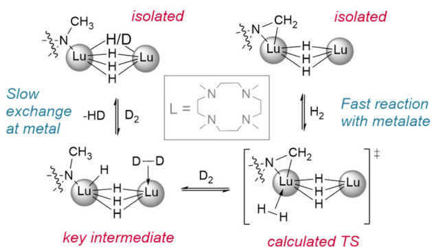
Fig. 3 Demonstration of the reactivity of metalated ligands in the activation of H 2 . Deuteration studies show metal based H/D exchange is slow with the tetrahydrido dimer while the metalated trihydrido complex reacts with H 2 /D 2 quickly. L = Me 4 -TACD.†
