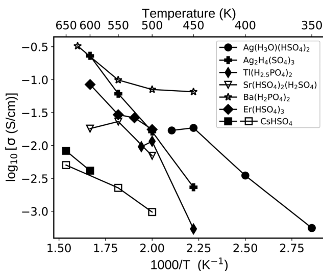
Fig. 7 Proton conductivities of selected solid acids calculated with AIMD (full symbols) and MLFF-AIMD (open symbols). The cell sizes and shapes were constrained to the room temperature (or low temperature) phases as retrieved from the Materials Project database (see Table 2). The simulated CsHSO 4 (mp-1192419) conductivity is shown as a baseline (MLFF-AIMD and AIMD demonstrate consistent results; see Section S1 in the ESI† for further details).
