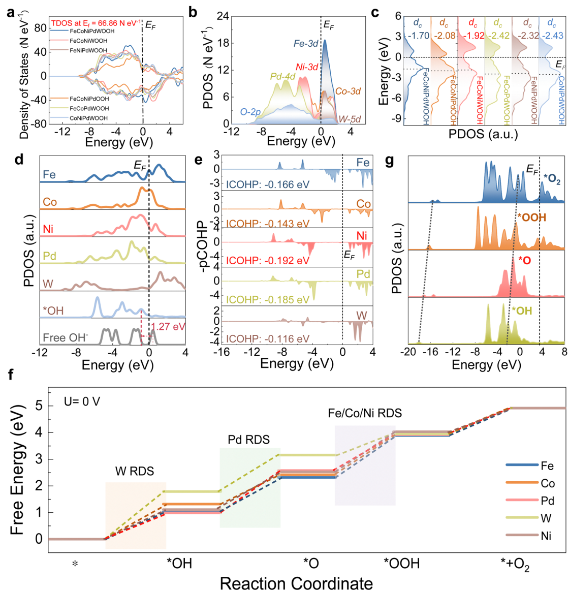
Fig. 4 DFT calculation results. (a) TDOS of FeCoNiPdWOOH, FeCoNiPdWOOH, FeCoNiPdWOOH, FeCoPdWOOH, FeNiPdWOOH, and CoNiPdWOOH. (b) PDOS of FeCoNiPdWOOH. (c) Electronic density of states of the d-band for the metal atoms in various models. (d) PDOS for OH adsorption at various active sites. (e) COHP bonding analysis of M–O interactions (M in the surface site over FeCoNiPdWOOH and O in adsorbed OH). (f) Standard free energy diagram of the OER process at 0 V of FeCoNiPdWOOH for various active sites. (g) PDOS of key intermediates over Ni sites in FeCoNiPdWOOH.
