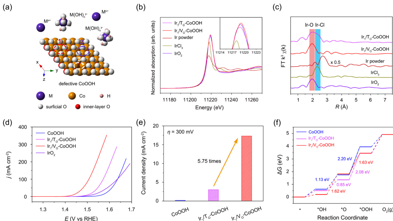
Fig. 6 (a) Schematic illustration of oxygen-terminated (001) surface of defective CoOOH with the single atom anchoring sites. (b) XANES and (c) FT-EXAFS spectra of Ir 1 /T 5 O-CoOOH, and Ir 1 /V 5 O-CoOOH, Ir powder, IrCl 3 , and IrO 2 . (d) Polarization curves of CoOOH, Ir 1 /T 5 O-CoOOH, and Ir 1 /V 5 O-CoOOH. (e) Specific activities of samples normalized by ECSA at an overpotential of 300 mV. (f) Free energy diagram of CoOOH, Ir 1 /T 5 O-CoOOH, and Ir 1 /V 5 O-CoOOH in OER. Reproduced with permission from ref. 49. Copyright 2022. Springer Nature.
