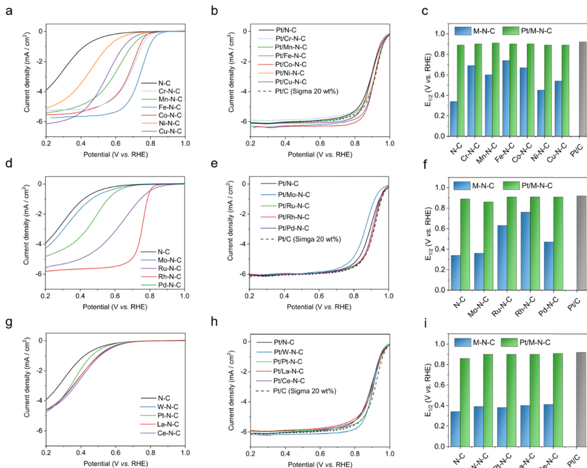
Fig. 4 ORR performance evaluated by RDE in 0.1 M \text{HClO}_4 with a scan speed of 5 \text{ mV s}^{-1} . (a)–(c) Half-wave potentials for bare M–N–C catalysts, Pt supported M–N–C (Pt/M–N–C) and summary of half-wave potentials for 3d metals. (d)–(f) Half-wave potential for 4d metals. (g)–(i) Half-wave potentials for 5d and f metals.
