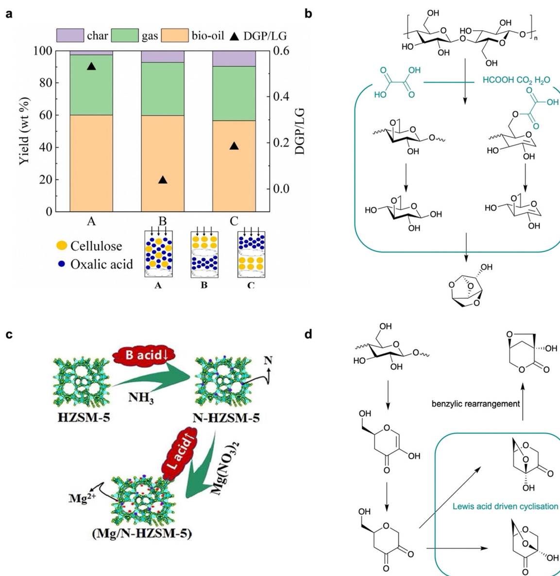
Fig. 4 (a) Performance comparison of cellulose CFP with oxalic acid to produce DGP in different loading set-ups. 18 (b) Reaction pathway of cellulose CFP to produce DGP. (c) Modification of HZSM-5 for cellulose CFP. 40 (d) Reaction pathway of cellulose CFP to produce LAC.
