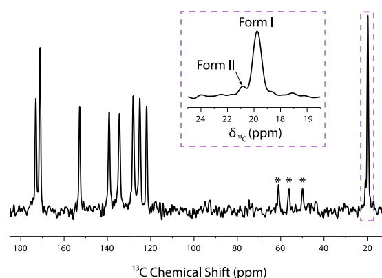
Fig. 4 T_{1\rho} -filtered ^{13}\text{C} CPMAS NMR spectrum recorded on a mesoporous SBA-15 silica material impregnated with a 0.8 M solution of aspirin in ethanol. This experiment was recorded 2 days after material impregnation, without microwave irradiation and at a temperature of 98 K. Signals labelled with "*" correspond to spinning side bands. The ^{13}\text{C} NMR chemical shift of the methyl group signal of forms I and II are at 19.8 ppm and 20.9 ppm, respectively.
