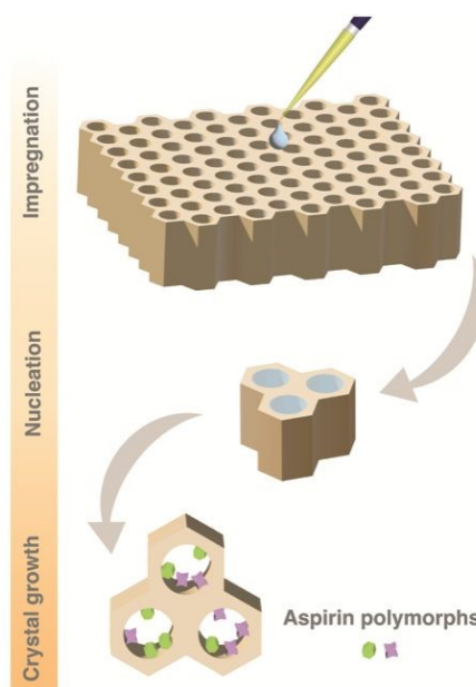
Fig. 1 Schematic representation of crystallisation of aspirin within the pores of mesoporous SBA-15 silica material (with or without wall-embedded TEMPO radicals). The mesoporous silica material is impregnated with a solution of aspirin in ethanol (0.8 M). Evaporation of solvent (ethanol) leads to crystallisation of aspirin within the pores of the material.
