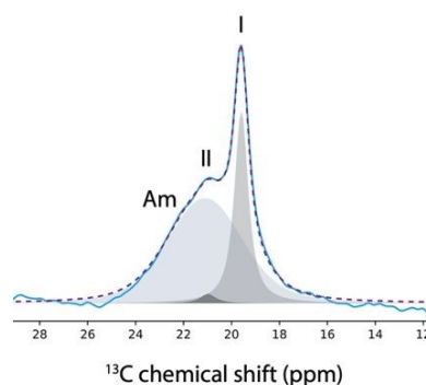
Fig. 3 ^{13}\text{C} NMR resonances corresponding to the methyl group of aspirin spectrum (blue curve) recorded at 98 K on a mesoporous SBA-15 silica material 2 days after impregnation with a solution of aspirin in ethanol (0.8 M). The Gaussian peaks used for the deconvolution are shown as filled grey shapes and their sum is shown as a dotted purple line. The 3 Gaussian peaks correspond to the individual ^{13}\text{C} NMR resonances of the amorphous phase (Am), and the crystalline phases of form I and II of aspirin.
