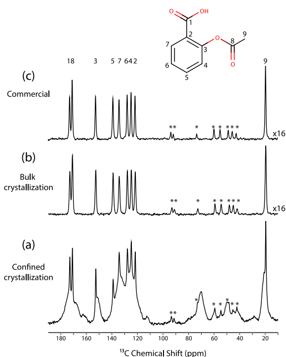
Fig. 2: (a) ^{13}\text{C} CPMAS NMR spectrum recorded for a mesoporous SBA-15 silica material without wall-embedded TEMPO radicals and impregnated at room temperature with a solution of aspirin in ethanol (0.8 M). The spectrum was recorded 2 days after impregnation. (b) ^{13}\text{C} CPMAS NMR spectrum recorded for a powder sample of aspirin subsequently obtained from a solution of aspirin in ethanol. (c) ^{13}\text{C} CPMAS NMR spectrum of commercial aspirin. All spectra were recorded without microwave irradiation and at a temperature of 98 K. Signals labelled with "*" correspond to spinning side bands.
