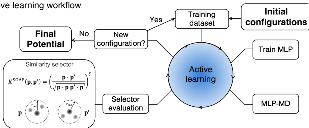
Fig. 1 Training data and active learning workflow: a) Training subsets for Mg 2+ in aqueous solution, b) training subset for Pd 2+ in acetonitrile (MeCN), c) Scheme of the active learning workflow used to train the machine-learning potentials (MLPs).
