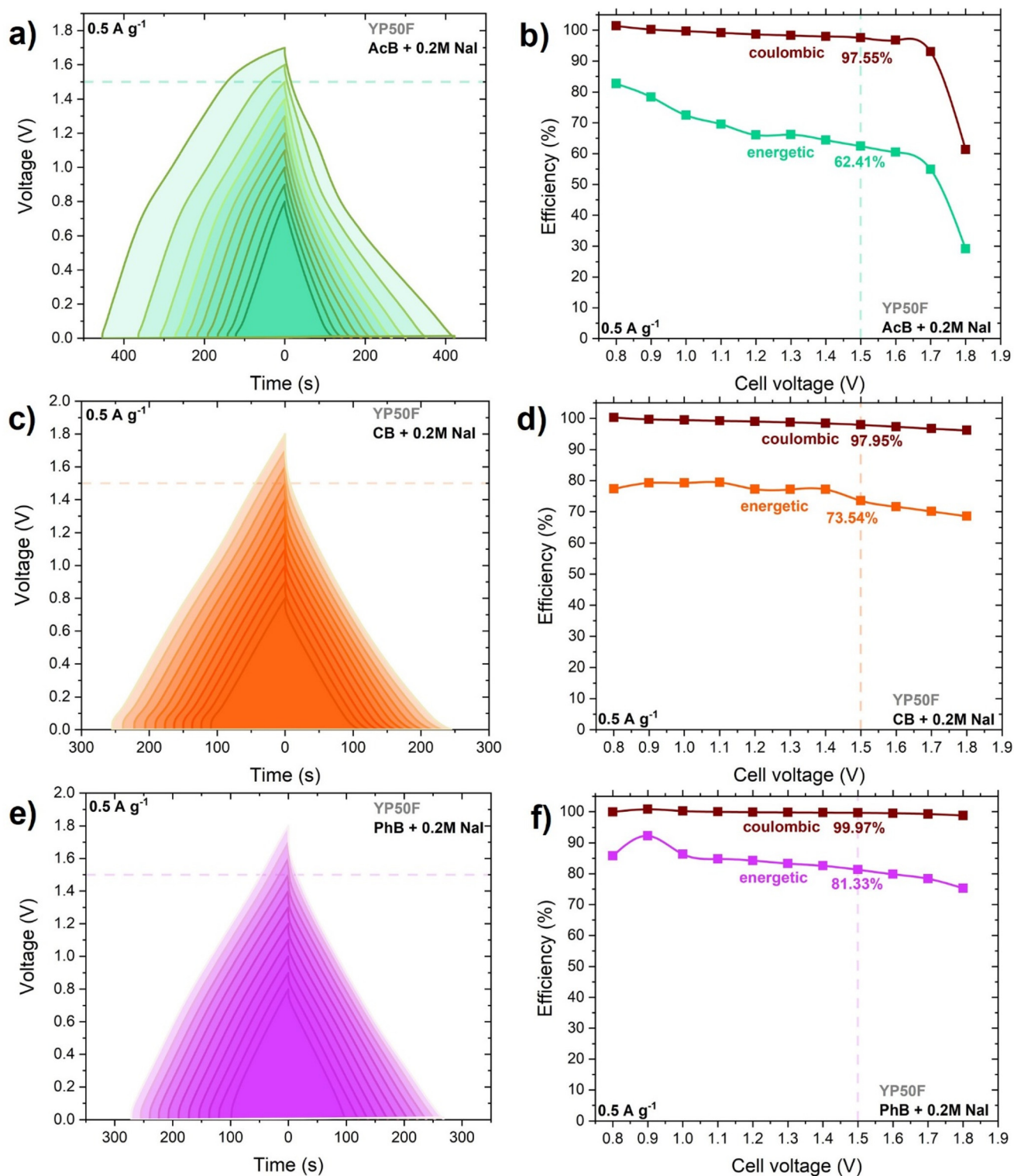
Fig. 2 Galvanostatic charge/discharge voltage extension at 0.5 \text{ A g}^{-1} for ECs operating in (a) acetate buffer + 0.2 \text{ mol L}^{-1} NaI, (c) citrate buffer + 0.2 \text{ mol L}^{-1} NaI, and (e) phosphate buffer + 0.2 \text{ mol L}^{-1} NaI for various voltages. Energetic and coulombic efficiency calculated from the GCD curves for ECs operating in (b) acetate buffer + 0.2 \text{ mol L}^{-1} NaI, (d) citrate buffer + 0.2 \text{ mol L}^{-1} NaI, and (f) phosphate buffer + 0.2 \text{ mol L}^{-1} NaI.
