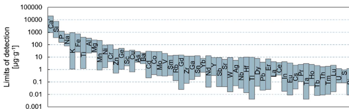
Fig. 2 Min–max range of limits of detection as obtained using LA-ICP-ToF-MS mapping of 0.004–0.05 mm 2 areas over a period of ~1 year. 2 μm ϕ circular, 3 μm ϕ circular, and 5 μm × 5 μm square laser spot sizes were used. Note that actual LoDs depend on multiple parameters other than the spot size. LoDs were calculated following Pettke et al. 20 Tuning of the mass analyzer may result in an improved sensitivity for the lower mass range, at the cost of sensitivity in the higher mass range.
