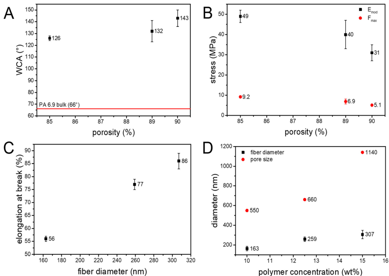
Fig. 2 Different membrane characteristics of the EFMs made from PA 6.9, (A) water contact angle (WCA) and (B) stiffness ( E_{\text{mod}} ) and ultimate tensile strength ( F_{\text{max}} ) in dependence of the porosity, (C) elongation at break against the fiber diameter and (D) fiber diameter and pore size against the polymer concentration.
