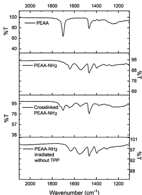
Fig. 2 A comparison of FTIR spectra of PEAA, PEAA-8C-NH 2 , crosslinked PEAA-8C-NH 2 , and PEAA-8C-NH 2 irradiated without photosensitizer. Similar spectra were observed for PEAA-3C-NH 2 , PEAA-6C-NH 2 , and PEAA-8C-NH 2 between 1100 and 2100 cm -1 .
