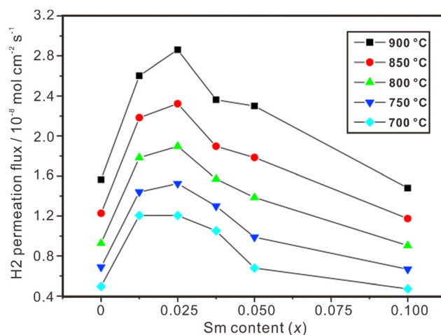
Fig. 11 Hydrogen permeation flux through \text{Ni}-(\text{La}_{1-x}\text{Sm}_x)_2\text{Ce}_2\text{O}_{7-\delta} membranes. Reprinted with permission, 121 Copyright [2010] Elsevier.
