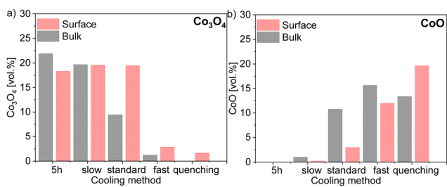
Fig. 11 Volume fraction of 60CGO20–FCO composite subjected different heat treatment and cooling methods in (a) \text{Co}_3\text{O}_4 and (b) CoO amount comparison in the bulk and surface.
