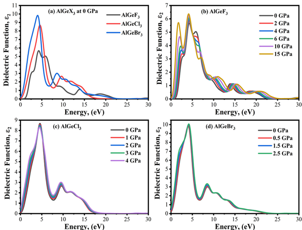
Fig. 7 Comparison of the imaginary part of the dielectric constant without pressure (a) \text{AlGeX}_3 ( X = \text{F}, \text{Cl}, \text{and Br} ) and with pressure (b) \text{AlGeF}_3 , (c) \text{AlGeCl}_3 , and (d) \text{AlGeBr}_3 .
