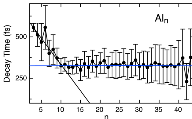
Fig. 3 Excited state lifetimes of \text{Al}_n ( n = 3\text{--}43 ) decrease with size for n < 10 , and then plateau for larger clusters reaching an average value of 327 fs. The black trend line corresponds to the fit of \text{Al}_3\text{--Al}_{10} , whereas the blue line is the fit of \text{Al}_{11}\text{--Al}_{43} .
