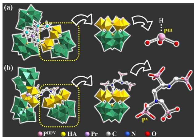
Fig. 3 Comparison of the inorganic HP III -inserted Dawson-like (HP III SeW 15 ) unit in 2a (a) and the organo-inorganic hybrid (C 6 N 2 P 4 SbW 15 ) unit in 1a (b).
