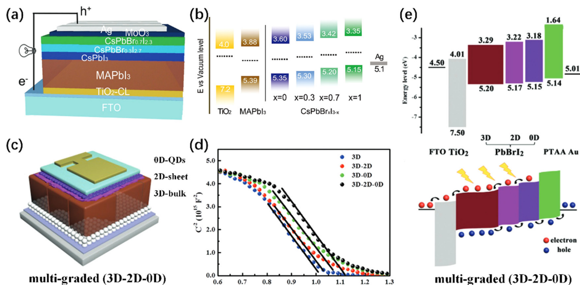
Fig. 10 (a) Schematic diagram of solar cell configuration with graded \text{CsPbBr}_x\text{I}_{3-x} films. (b) Energy diagram of solar cells with graded \text{CsPbBr}_x\text{I}_{3-x} . Copyright 2017, Wiley. (c) Schematic diagram of the gradient structure of the 3D–2D–0D perovskite. (d) Mott–Schottky curves with/without dimensional gradient heterojunctions. (e) Energy-level diagram of multigrade \text{CsPbBrI}_2 PSCs (top) and the carrier-transport mechanism in multigrade \text{CsPbBrI}_2 PSCs (bottom). 78 Copyright 2018, Wiley.
