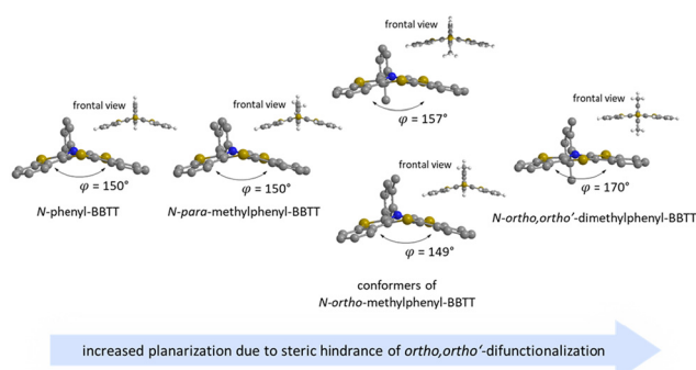
Fig. 2 Visualization of sterically restricted BBTTs due to the introduction of sterically demanding ortho,ortho' -substitution pattern (B3LYP/6-311++G**, IEFPCM \text{CH}_2\text{Cl}_2 ).
