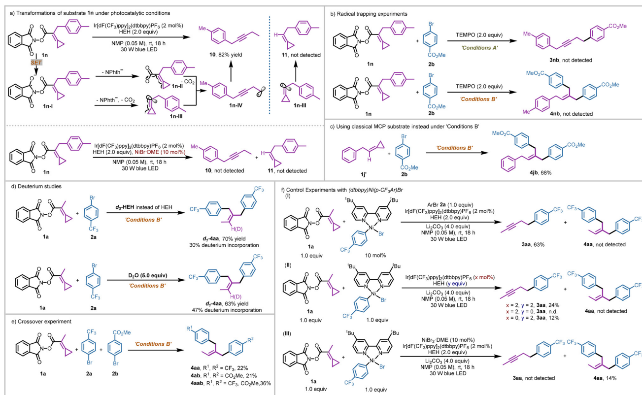
Scheme 6 Control experiments.
