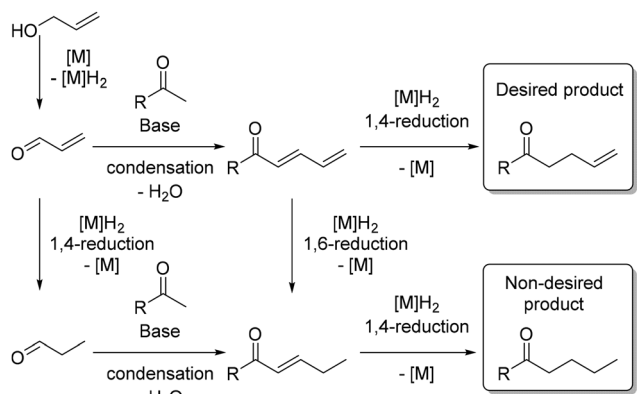
Scheme 82 Challenges associated with using allylic alcohols as pro-electrophiles.
