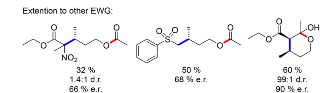
Scheme 77 Insertion of allylic alcohol in 1,3-diketones.
