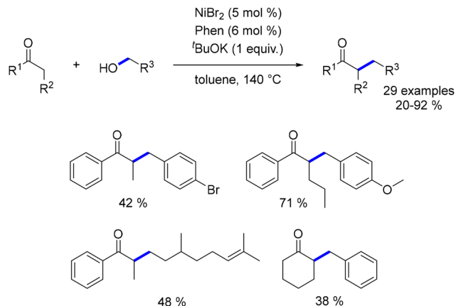
Scheme 101 Alkylation of α-substituted ketones.
