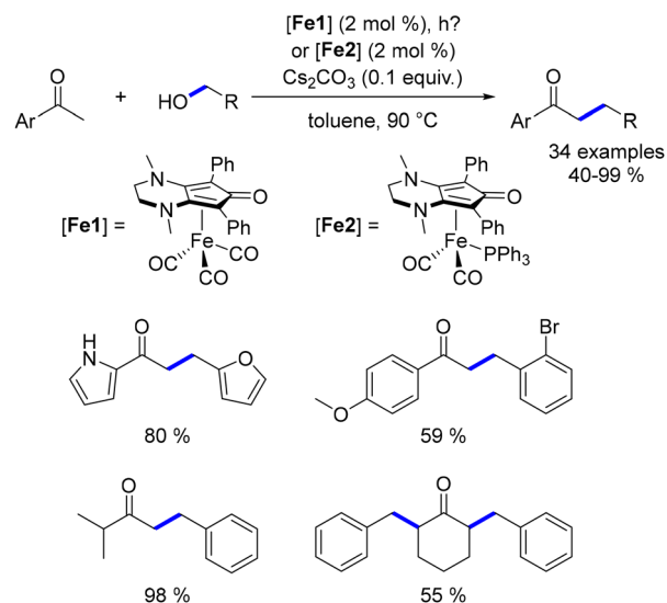
Scheme 80 Alkylation of ketones, as reported by Renaud.
