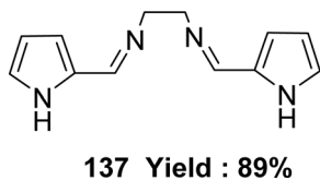
Fig. 55 Structure of Schiff base ligand 137.
