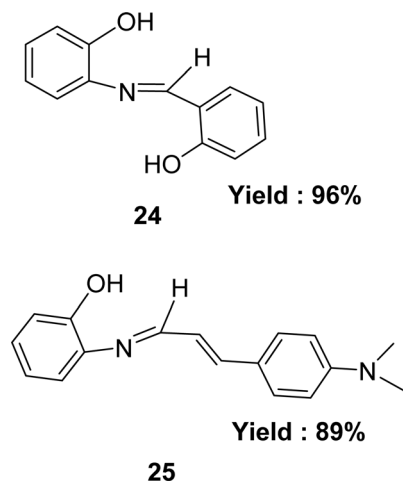
Fig. 17 Structure of Schiff base ligands 24 and 25.
