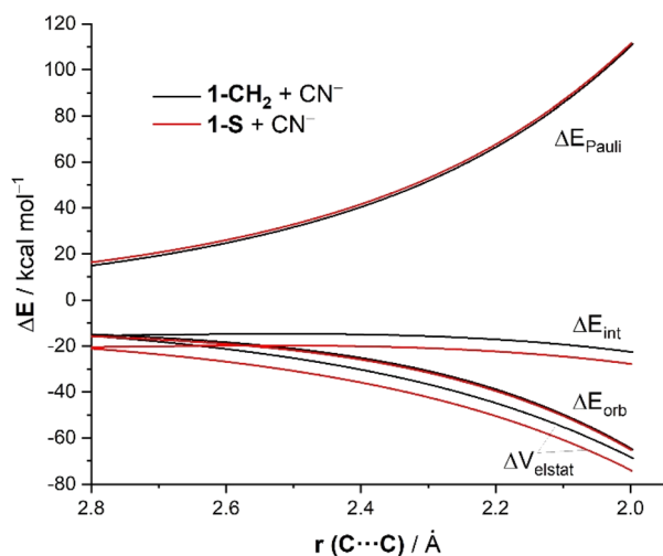
Fig. 2 Comparative EDAs of the reaction between \text{CN}^- and 1-CH 2 or 1-S projected onto the C...C bond-forming distance and referred to the isolated reactants. All data have been computed at the ZORA-M06-2X/TZ2P//M06-2X/6-311+G* level.
