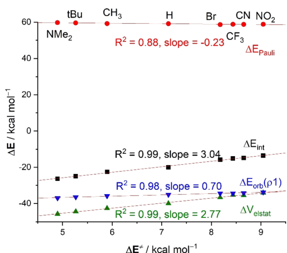
Fig. 6 Plot of the activation energies ( \Delta E^\ddagger ) and the EDA terms for the reactions of \text{CN}^- and benzaldehydes 2 (at a consistent \text{C}\cdots\text{C} bond-forming distance of 2.232 Å). All data have been computed at the ZORA-M06-2X/TZ2P//M06-2X/6-311+G* level.
