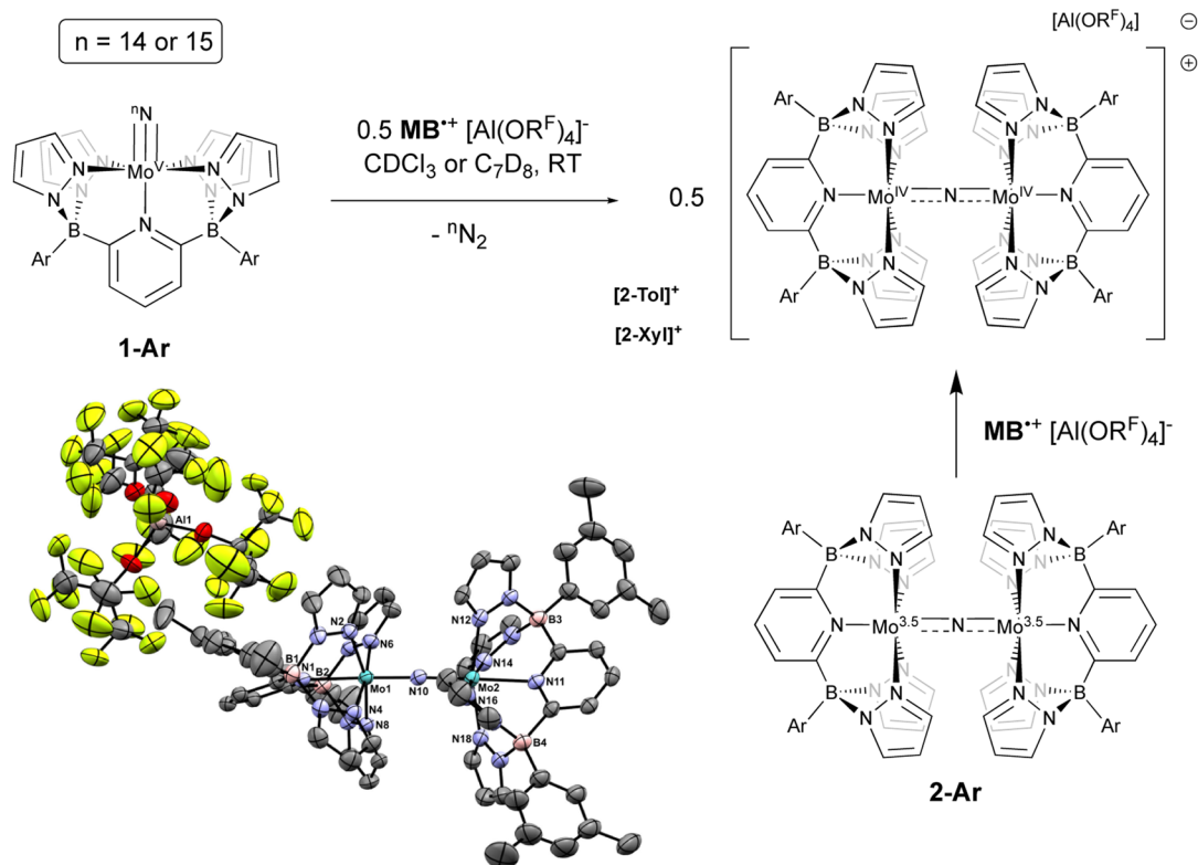
Fig. 3 Oxidation of neutral nitridos 1-Ar with 0.5 equivalents of [\text{MB}]^+[\text{Al}(\text{OR}^F)_4]^- . Lower left: molecular structure of [\mathbf{2-Xyl}]^+[\text{Al}(\text{OR}^F)_4]^- . Thermal ellipsoids are shown at the 50% probability level and all H atoms are omitted for clarity. Selected bond distances (Å): Mo(1)–N(10), 1.856(3); Mo(2)–N(10), 1.859(3); Mo(1)–N(1), 2.260(3); Mo(2)–N(11), 2.265(3). Selected bond angles (°): Mo(1)–N(10)–Mo(2), 176.52(19).
