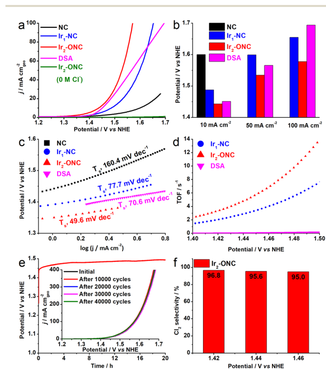
Fig. 3 Electrocatalytic CER performance of \text{Ir}_2\text{-ONC} and other control samples. (a) LSV polarization curves, recorded at a scan rate of 5 \text{ mV s}^{-1} in 0.1 \text{ M HClO}_4 + 4 \text{ M NaCl} . (b) Comparison of the overpotentials of different samples to reach 10, 50 and 100 \text{ mA cm}^{-2} . (c) Tafel slopes. (d) Calculated TOFs of \text{Ir}_1\text{-NC} , \text{Ir}_2\text{-ONC} and DSA. (e) Chronopotentiometric curves of \text{Ir}_2\text{-ONC} , recorded at a constant current density of 10 \text{ mA cm}^{-2} in 0.1 \text{ M HClO}_4 + 4 \text{ M NaCl} . The inset shows the cyclic durability. (f) CER selectivity of \text{Ir}_2\text{-ONC} at different potentials.
