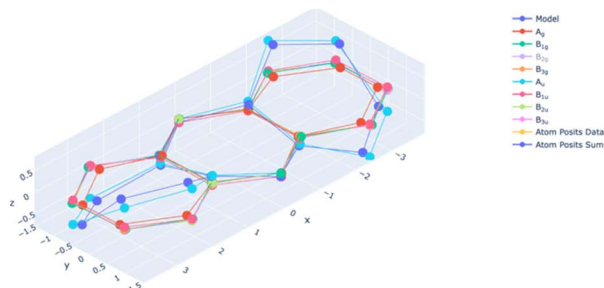
Figure 2: Atom positions and symmetric decomposition modes
