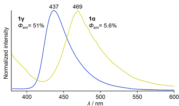
Fig. 5 Emission spectra of 1α and 1γ under excitation at 365 nm.
