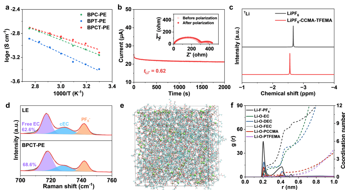
Fig. 3 (a) Ionic conductivity fitted using Arrhenius plots for BPC-PE, BPT-PE and BPCT-PE. (b) Current–time profile for the \text{Li}|\text{BPCT-PE}|\text{Li} cell at 10 mV of polarization (inset: Nyquist plots before and after polarization). (c) ^7\text{Li} NMR spectra of \text{LiPF}_6 and \text{LiPF}_6 -CCMA-TFEMA in \text{CD}_3\text{CN} . (d) Raman spectra of LE and BPCT-PE. (e) A snapshot of the MD simulation box for BPCT-PE. (f) Radial distribution functions (solid lines) and corresponding coordination numbers (dashed lines) of BPCT-PE.
