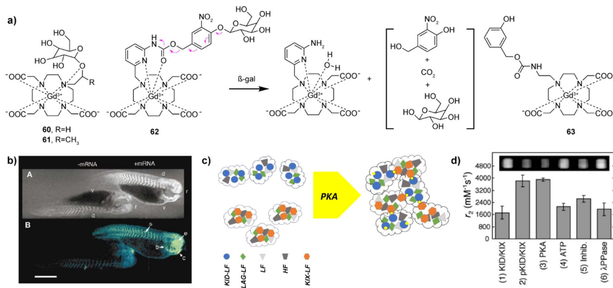
Fig. 9 Enzyme responsive MRI probes. (a) The structures of enzyme-sensitive MRI probes 60 – 63 . (b) MR images of two embryos injected with probe 61 at the two-cell stage (top), while the embryo on the right was also injected with \beta -gal mRNA. Consequently, the signal strength is 45–65% greater in the embryo on the right that contains \beta -gal; pseudocolor rendering of the same image (top) with water made transparent (bottom). (c) Schematic illustration of the self-assembly and aggregation processes of NP-KID-FtNs in response to PKA activity. Genes encoding Ft are premixed and co-transfected into cells, where proteins are expressed and spontaneously assembled into KID-FtNs and KIX-FtNs (left). KID-LF chains are phosphorylated by PKA to form pKID-LF. Modified KID-FtNs (pKID-FtNs) containing pKID-LF form supramolecular aggregates with KIX-FtNs, which affect the MRI signal (right). (d) Measurements of the transverse relaxivity of Ft-based NP sensors in response to PKA activity. Incubation of the sensor (3 : 2 ratio of KID-FtNs with KIX-FtNs) with PKA for 2 h roughly doubled the r_2 relaxivity. Adapted with permission from: (b) ref. 114 Copyright © 1969, Springer Nature, and (d) ref. 125 Copyright © 2009 American Chemical Society.
