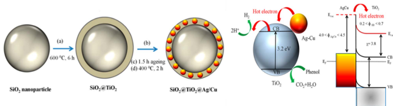
Fig. 29 Schematic and possible pathway for enhanced photocatalysis in the hybrid SiO 2 @TiO 2 @Ag-Cu core-shell structure. Reproduced with permission. Copyright 2020 American Chemical Society. 142
