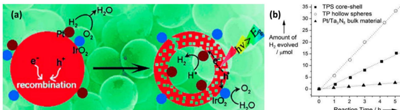
Fig. 28 (a) \text{Ta}_3\text{N}_5 core/shell photocatalyst deposited with Pt and \text{IrO}_2 . (b) Periodic evolution of \text{H}_2 on hollow spheres, core/shell particles, and a bulk \text{Ta}_3\text{N}_5 photocatalyst. Reproduced with permission. Copyright 2013 Wiley. 270
