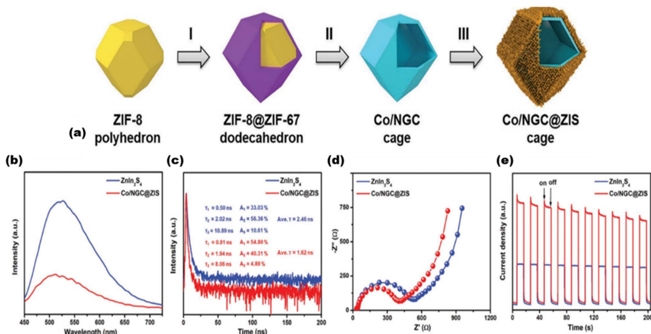
Fig. 30 (a) Diagram illustrating the formation of hierarchical Co/NGC@ZIS cages. (b) Steady-state photoluminescence data. (c) Time-resolved photoluminescence data. (d) Electrochemical impedance spectroscopy data. (e) Transient photocurrent spectra. Reproduced with permission. Copyright 2019 Wiley. 194
