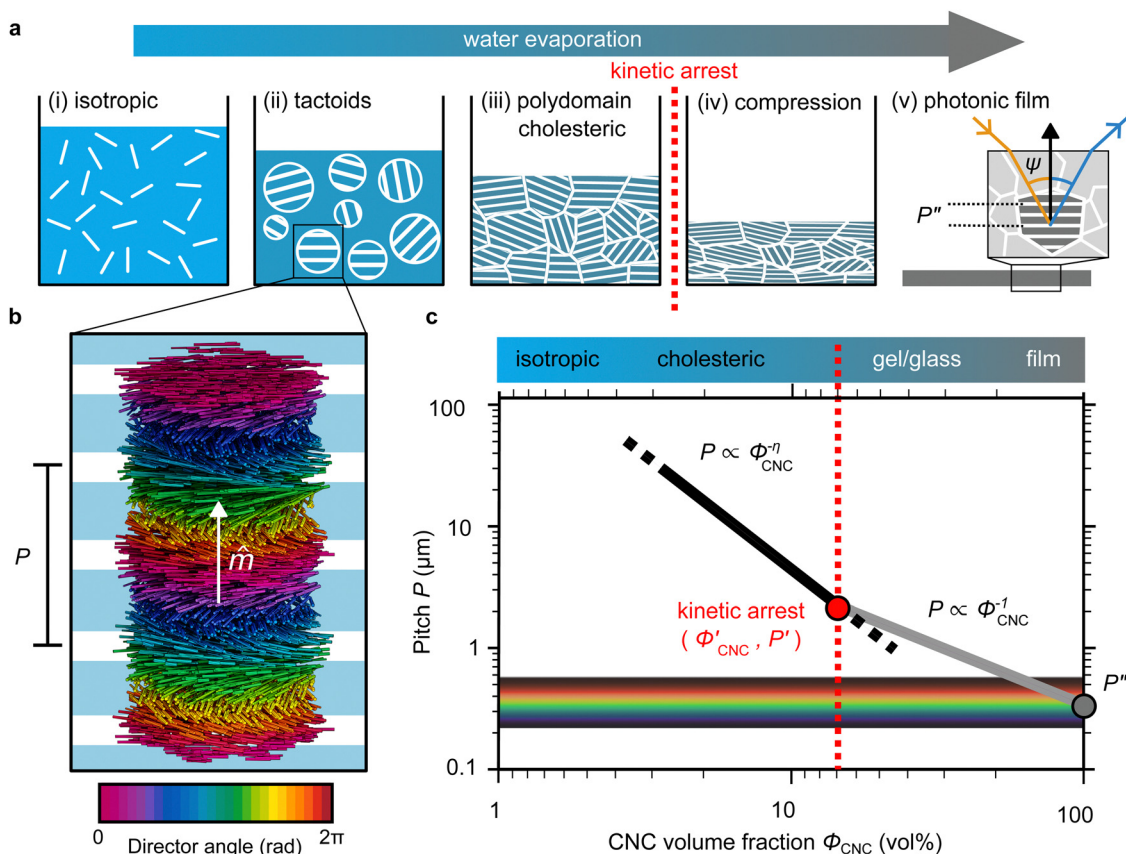
Fig. 1 (a) Schematic (not to scale) illustrating the evolution of the CNC suspension upon drying, showing (i) the initial isotropic phase, (ii) formation of tactoids leading to (iii) a polydomain cholesteric texture that is fixed by kinetic arrest. (iv) Further geometric compression of the structure results in (v) a helicoidally structured film with structural colour. (b) Rendering of rod-like particles in a left-handed helicoidal structure. The helical axis vector, \hat{m} , and pitch, P , are indicated. Rod colour indicates local director angle, while the underlying white stripes represent the P/2 periodicity of the “fingerprint pattern” observable by optical microscopy. (c) Expected pitch evolution with CNC volume fraction for an aligned helicoidal domain, exhibiting two regimes with different power-law exponents, with a transition at the point of kinetic arrest ( \Phi'_{\text{CNC}}, P' ) and resulting in a final pitch P'' in the visible regime, as indicated by the rainbow band.
