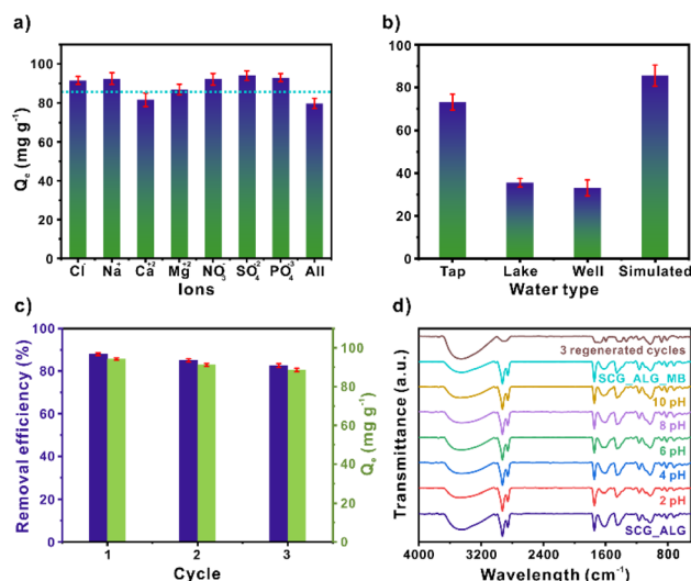
Fig. 7 (a) Ion influence for MB adsorption over SCG_ALG ([MB] = 50 \text{mg L}^{-1} ; SCG_ALG = 10 mg, volume = 20 ml, time = 180 min, pH = 6, room temperature); (b) MB adsorption using SCG_ALG as an adsorbent in deionized (DI) water and water from natural sources (tap water, well water, and lake) ([MB] = 50 \text{mg L}^{-1} ; SCG_ALG = 10 mg, volume = 20 ml, time = 60 min, room temperature); (c) regeneration studies for MB adsorption over SCG_ALG ([MB] = 50 \text{mg L}^{-1} ; SCG_ALG = 10 mg, volume = 20 ml, time = 180 min, pH = 6, room temperature); (d) FT-IR spectra of water stability at 2–10 pH interval of SCG_ALG, after adsorption, and regeneration experiments.
