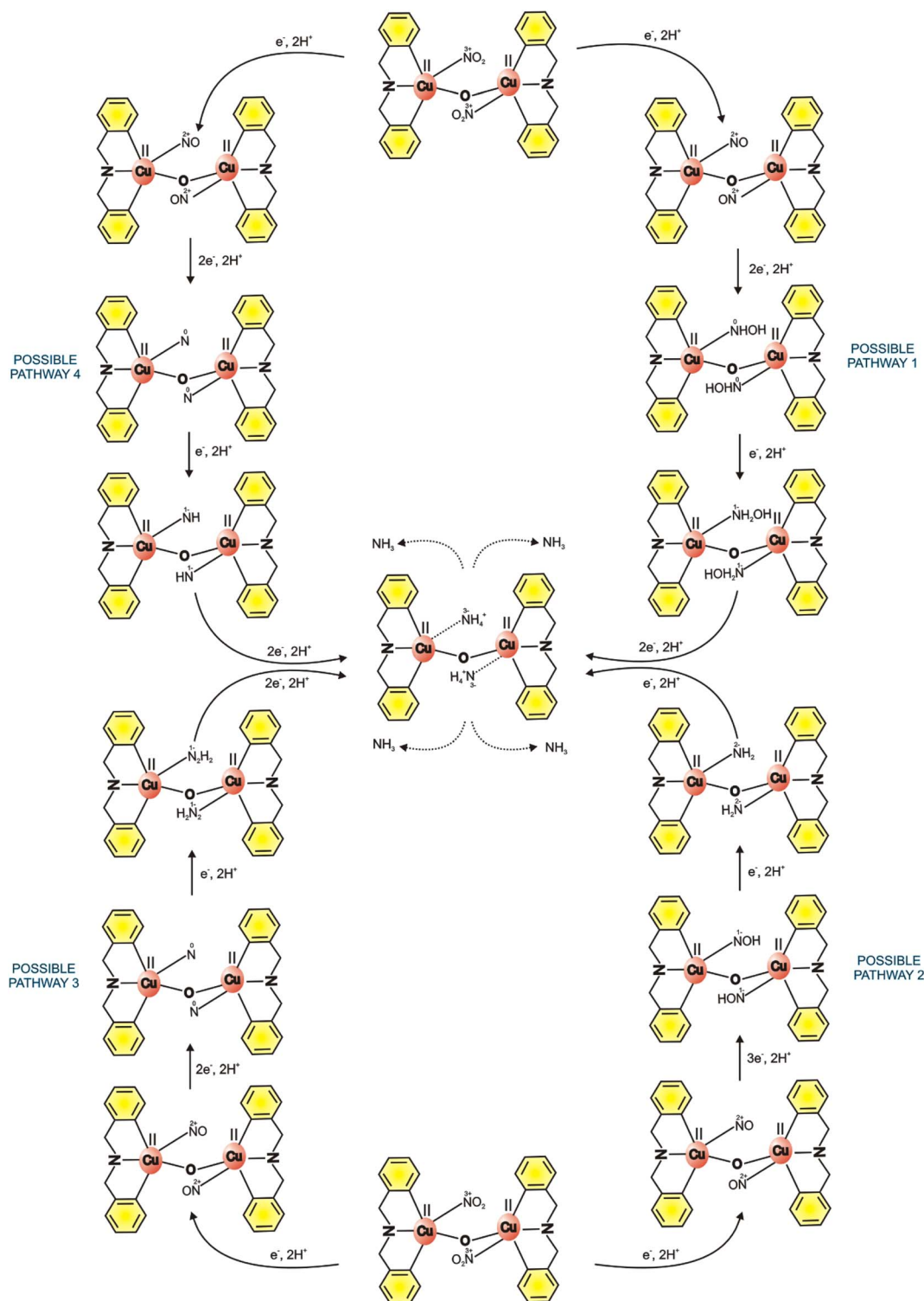
Scheme 3 Possible electrochemical reduction reaction mechanism pathway of \text{GMC@Cu}_2(\mu\text{-O})_2 on nitrite to form ammonium. The adsorbed \text{NO}_2^- is first reduced to \text{NO} and its conversion to \text{NH}_3 occurs via four pathways: pathway 1: \text{NO} \rightarrow \text{NHOH} \rightarrow \text{NH}_2\text{OH} \rightarrow \text{NH}_3 ; pathway 2: \text{NO} \rightarrow \text{NOH} \rightarrow \text{NH}_3 ; pathway 3: \text{NO} \rightarrow \text{N} \rightarrow \text{NH}_3 ; pathway 4: \text{NO} \rightarrow \text{N} \rightarrow \text{NH} \rightarrow \text{NH}_3 . The oxidation states of nitrogen are depicted at each step.
