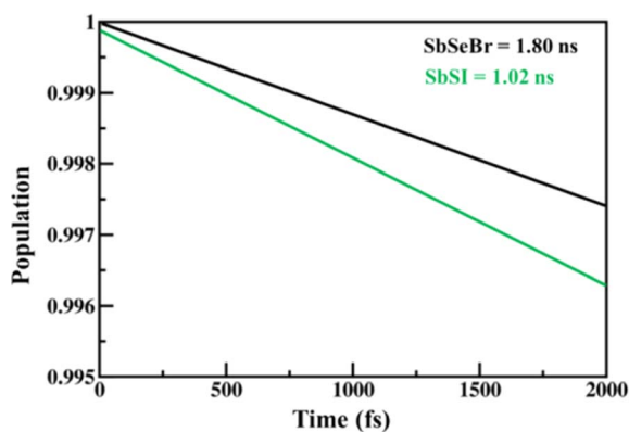
Fig. 12 The electron–hole recombination dynamics of 2D Janus SbSI and SbSeBr monolayers.
