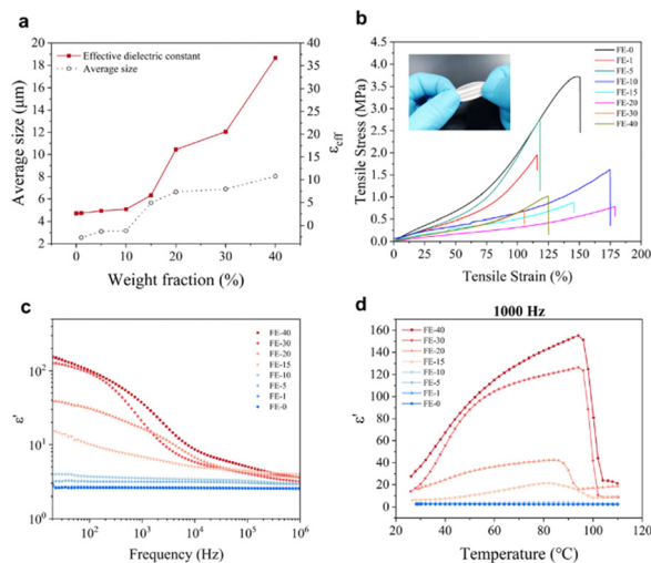
Fig. 2 (a) Average size of N_F LC droplets and effective dielectric constant (at 25 ^{\circ}\text{C} 1 kHz) versus N_F LC weight fraction in FE composites. (b) Stress–strain curves of FE composites with different N_F LC weight fractions. (c) The spectrum of the real part of the complex dielectric constant of FE composites with different N_F LC weight fractions at room temperature. (d) The real part of the complex dielectric constant versus temperature for different N_F LC weight fractions.
