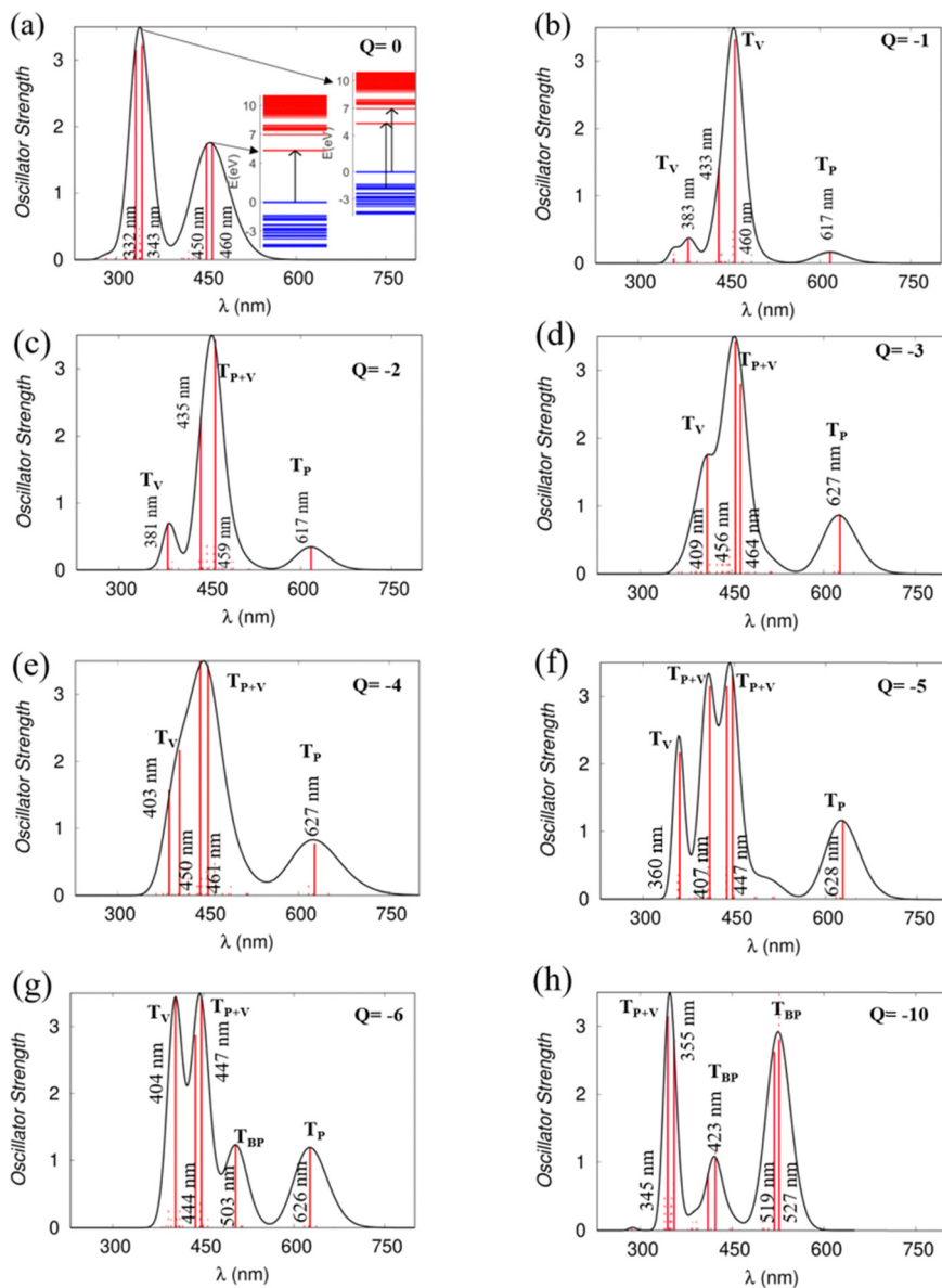
Fig. 7 UV vis/NIR absorption spectra of (a) the charge neutral PNDI-TVTV chain and (b)–(h) the doped PNDI-TVTV chain at various charged states from Q = -1 to -6 and -10 indicating the corresponding electronic transitions calculated in the solvent phase.
