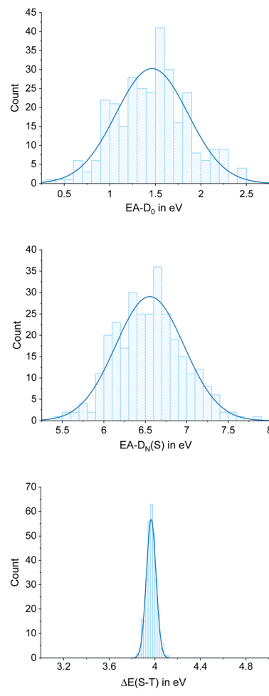
Fig. 5 Electron attachment energy calculated using the charge stabilization method at the EOM-EA-CCSD/cc-pVDZ/EFP level, for (a) the first 1p resonance, EA-D_0 , and (b) the first 2p1h resonance, EA-D_{N(S)} . (c) Singlet-triplet gap, \Delta E(S-T) , distribution at the EOM-EA-CCSD/cc-pVDZ/EFP level.
