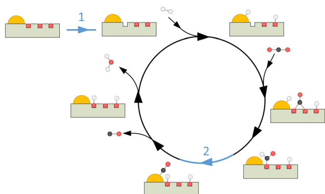
Fig. 8 Proposed associative monobridged formate-mediated reaction mechanism for the plasmonic-driven rWGS reaction over Au/ \text{CeO}_{2-x} upon illumination. In fully oxidised catalysts, the rate-determining step (blue 1) is the plasmonic-driven generation of vacancies near Au NPs. For catalysts with a reducing treatment, the rate-determining step (blue 2) is proposed to be the dissociation of the formate intermediate. Atoms are labelled as Au (gold), C (black), H (white), O (red).
