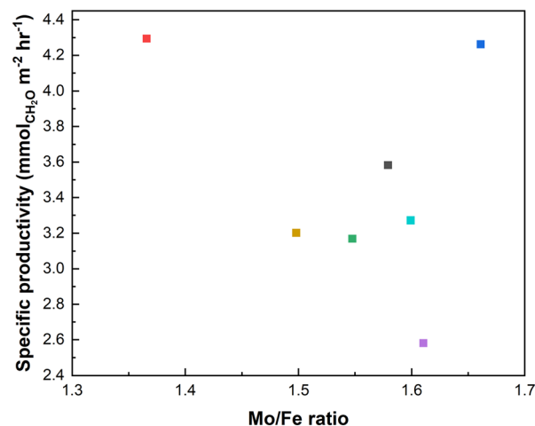
Fig. 5 Specific productivity of \text{CH}_2\text{O} in relation to Mo/Fe ratio.
