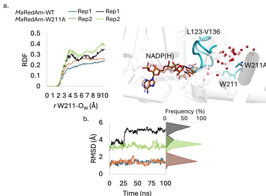
Fig. 3 RDFs of the W211- O_w pair calculated from molecular dynamics (MD) simulations (a) and RMSD of the L123-V136 loop (b) obtained from MaRedAm -WT and MaRedAm -W211A systems. For clarity, hydrogens were omitted, and only relevant species were reported. Atoms in the transparent background are those of the wild-type enzymes, while water molecules are depicted as red spheres.
