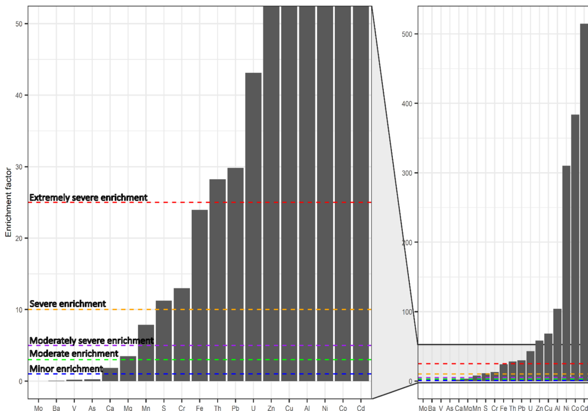
Fig. 3 Enrichment factors (EF) for elements measured in water from the precipitation pond of the Taraldrud site. Colored dashed lines indicate threshold levels for enrichment classification (i.e., minor, moderate, moderately severe, severe, and extremely severe enrichment). EF for Cr, Cu, Zn, Cd, and Pb were calculated using the limit of detection for the method.
