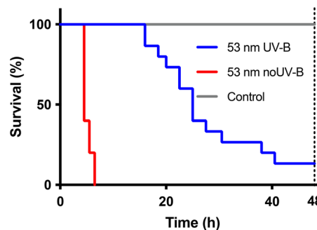
Fig. 4 Acute toxicity test with 53 nm amine-modified polystyrene particles. Kaplan-Meier survival curves for D. magna exposed to UV-B exposed (blue line) and UV-B shaded (red line) nanoplastics. The grey line shows a control treatment only containing water. Total exposure time is 48 hours as highlighted by the dotted vertical line.
