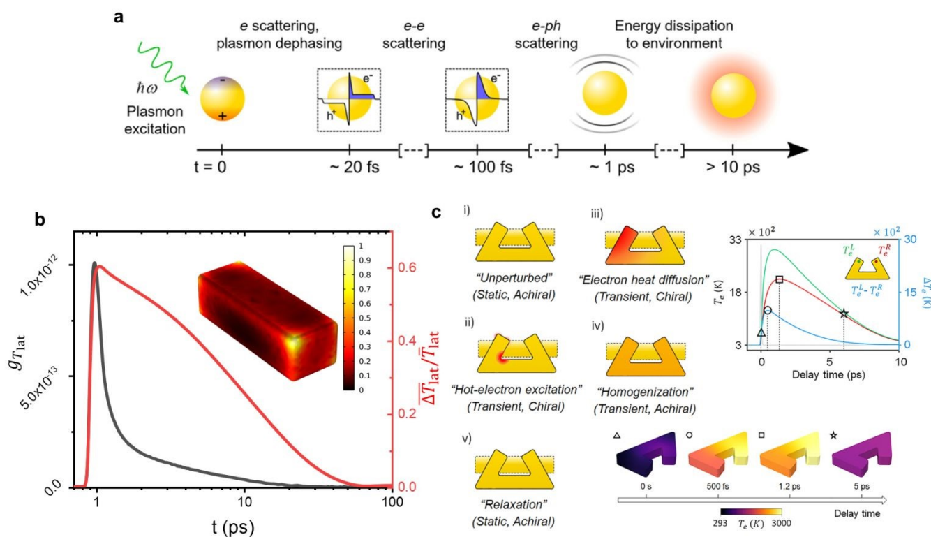
Figure 13. (a) Schematic diagram depicting significant stages and approximate timescales involved in the transfer of energy from the highly ordered collective oscillation of electrons in a plasmon, to single-particle states, to then the lattice and finally dissipating when heating the local environment. (b) Computational results showing timescales for two types of surface inhomogeneity on the lattice temperature of a gold nanoprism: chiral asymmetry and temperature inhomogeneity, as defined in the text. The inset shows the normalized surface temperature after being illuminated with a RCPL pulse at 682 nm, at the time of maximum gT_{lat} , at t \sim 1 ps. (c) (i-v) Schematic diagram of the transient optical response, indicating in different shades of red the excited state of local electronic states, and labelling the different stages with notable phenomena and their properties. (Right) Computational data showing the transient values of the electronic temperature, T_e , after pumping with CPL. (Top) Plot indicating T_e at both extremes of the structure, as well as their difference. (Bottom) Surface maps of T_e for the resonator at four selected times, with symbol legend shared with the data in the top panel. Panel a was reproduced from Ref. 198. Panel c was reproduced from Ref. 220.
