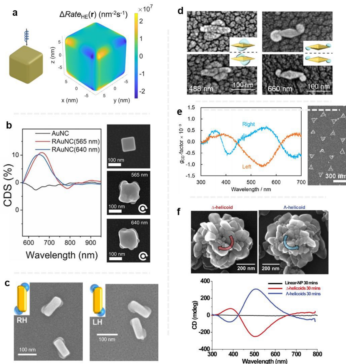
Figure 11. (a) Schematic diagram of the planar illumination condition for a Au nanocube, with the nanoparticle being illuminated from a fixed direction, and map of the differential rate of intraband hot carrier excitation under both polarizations of CPL. (b) Wavelength-dependent plasmon-induced chiral growth of AuNCs, including SEM images of a 100 nm-sized AuNC seed and equivalent nanoparticles after growth under RCP illumination at 565 nm and 640 nm, with the single-particle scattering CD spectra of these three NC. (c) SEM images, of Au nanoprisms with PbO 2 grown following chiral patterns under broadband CPL light of opposite handedness. The insets show 3D diagrams of the resulting metal-dielectric chiral hybrids. (d) SEM images of Au bipyramids with PbO 2 grown following chiral patterns under CPL with wavelengths of 488 nm (left) and 660 nm (right), resulting from illumination with opposite CPL polarization. Insets show 3D diagrams of the chiral hybrids. (e) Dissymmetry factor of the Ag metasurface (SEM image in right) after illumination with CPL with opposite polarizations in the 600 nm to 700 nm wavelength band. (f) SEM images of the nanohelicoids grown under LCPL (Δ) and RCPL (Λ), together with their CD spectra contrasted with that of pillars grown under LPL. Panel a was reproduced from Ref. 55. Panel b was adapted from Ref. 204. Panel c was adapted from Ref. 54. Panel d was adapted from Ref. 203. Panel e was adapted from Ref. 205. Panel f was adapted from Ref. 206.
