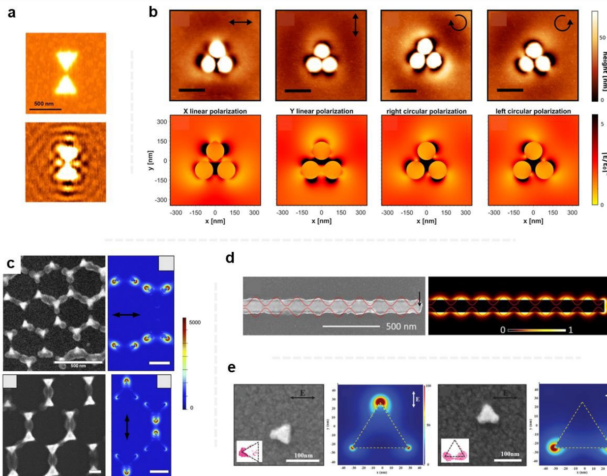
Figure 10. (a) Atomic force microscopy (AFM) images of a silver bowtie dimer after spin coating of polymer, before (top) and after (bottom) irradiation with light polarized orthogonally to the dimer major axis. (b) Gold trimer after polymer deposition and illumination with differently polarized light beams (polarization noted by the black symbols in top row). The top row shows AFM images, while the bottom row shows near field maps obtained from numerical simulations. Scale bars are 300 nm. (c) Scanning electron microscopy (SEM) images (left) of gold metasurface after driving 2-photon polymerization with light polarized along the horizontal (top) and vertical (bottom) axes, accompanied by maps of quadratic near field enhancement, |\mathbf{E}(\mathbf{r})|^2/E_0^2 , from numerical simulations (right). Scale bars without label are 200 nm. (d) Standing plasmon mode in a silver nanowire 2 \mu\text{m} long, showing a SEM image (left) excited by light polarized along its length after driving 2-photon polymerization around it, and with a map of normalized electric field from numerical simulations (right). (e) Au nanotriangles excited with different orientations relative to linearly polarized light. The SEM images show the nanotriangles and the hydrogel coalesced at their hot spots, while the accompanying panels show in field enhancement maps, |\mathbf{E}(\mathbf{r})|/E_0 , from numerical simulations. Panel a was adapted from Ref. 186. Panel c was adapted from Ref. 188. Panel d was adapted from Ref. 189. Panel e was adapted from Ref. 191.
