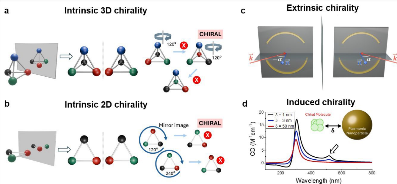
Figure 1. Types of chirality with example geometries. (a) Objects with intrinsic 3D chirality cannot be superimposed over their mirror images through any translation and rotation in 3D space. (b) Objects with intrinsic 2D chirality have the same property if we restrict the possible transformations to those within the plane of the object. (c) Extrinsic chirality arises when an achiral 2D object is excited by light at angle such that the combined system of object plus light is chiral in 2D. (d) Chirality induced on a plasmonic nanoparticle by closing its distance to a chiral molecule. The plot shows the CD of the whole system where \delta is the gap, in nm, between the nanoparticle and molecule.
