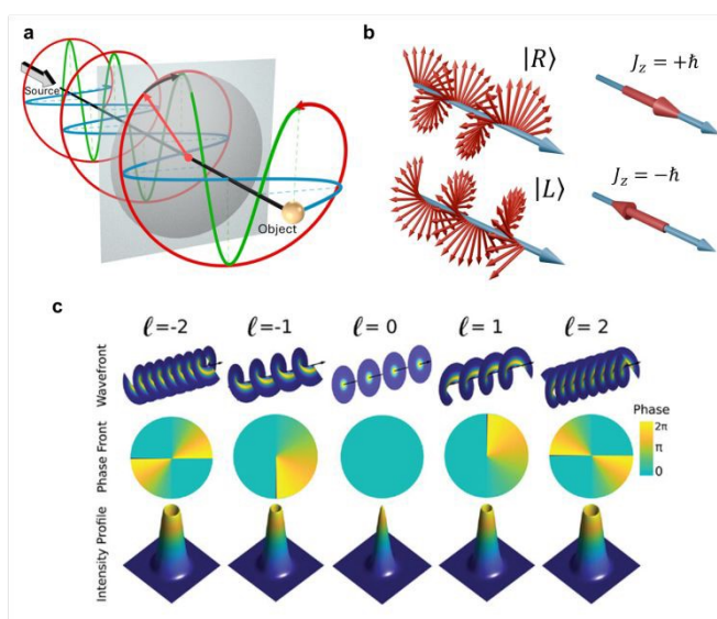
Figure 2. (a) Schematic diagram of a CP wave and the two LP waves composing it, with time fixed. Both source and object are labelled to indicate the two distinct perspectives that give rise to the two naming conventions for the handedness of CPL. In this example, the source (object) sees a counterclockwise (clockwise) rotation in the highlighted plane as time advances, so that it corresponds to LCPL (RCPL). (b) Photons are circularly polarized. (Left) Schematic diagrams of the rotating electric field at a fixed time, labelled with the handedness of the state in the source convention. (Right) Corresponding helicity, i.e. projection of the magnetic moment (from spin) over the propagation direction, of the photons with opposite handedness. (c) Vortex beams with orbital angular momentum. Intensity and phase profiles for the primary mode of a Laguerre–Gaussian beam with l = [-2, -1, 0, 1, 2] . The top row shows the phase front for the different modes. The middle row shows the corresponding azimuthal phase profiles, and the bottom row shows the corresponding planar intensity profile. Reproduced from Ref. 97.
