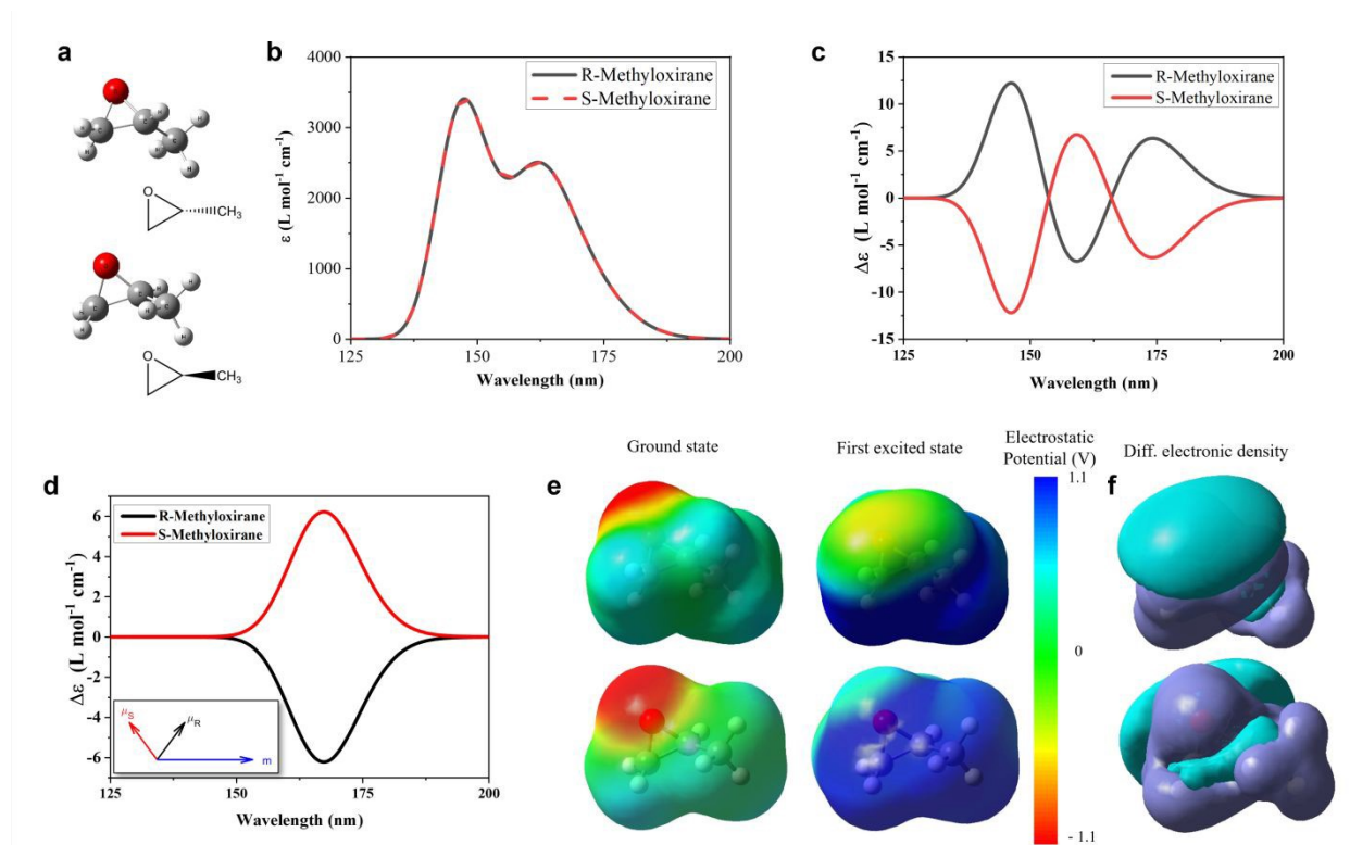
Figure 5. Numerical results for ab initio simulations of methyloxirane, or propylene oxide enantiomers. (a) Ball-stick 3D models of both enantiomers, accompanied by their Lewis structure diagrams. (b) Molar extinction coefficient of both enantiomers. Their spectra are indistinguishable at this scale. (c) Circular dichroism of both enantiomers. (d) Circular dichroism of the individual optical transition connecting the ground state with the first excited state. Inset: electric and magnetic transition dipole moments for both enantiomers, rotated so that \mu_s and \mu_R overlap and the projection of \mu_s and \mu_R are clearly shown to be equal and opposite, and thus R_s = -R_R . (e) Maps of the electrostatic potential surrounding the R-methyloxirane (top) and S-methyloxirane (bottom) at both their ground state and first excited state. The maps are plotted on isosurfaces of electronic density. (f) Two isosurfaces, with positive (turquoise) and negative (purple) values, of the difference of electronic density between the first excited state and ground state for both enantiomers.
