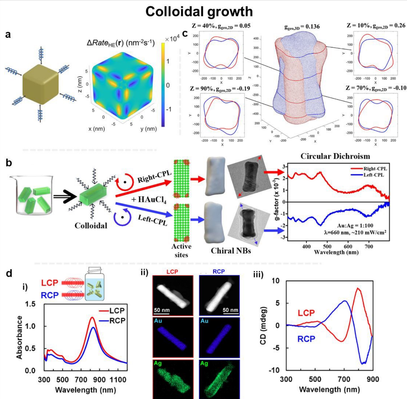
Figure 12. (a) Schematic diagram of the model for continuous CPL illumination of a colloidal Au nanocube, with the effective response being an average of six different directions for the propagation of light, and map of the differential rate of intraband hot carrier excitation under both polarizations of CPL. (b) Scheme of transformation of achiral nanobars into chiral ones in a colloidal suspension, driving galvanic replacement reaction (GRR) CPL illumination of colloidal Au@Ag nanoprisms, alongside 3D models of the resulting geometries (obtained with TEM tomography), TEM images of the chiral bimetallic structures, and dissymmetry factor of the sample after illumination with CPL at 660 nm. (c) Geometrical analysis of the tomographic reconstruction of one of the resulting chiral structures (in blue), together with its mirror image (in red). Four transversal cross-sections of the geometries are shown. Quantitative measures of the geometric chirality of the nanostructure and its cross-sections are also shown. (d) Photodeposition of Ag over Au nanorods under 630 nm light. (i) Absorbance of the samples after 12 h of CPL illumination; (ii) STEM images of the chiral bimetallic samples, with energy-dispersive X-ray spectroscopy maps identifying elemental spatial distribution; (iii) CD spectra of the samples. Panel a was reproduced from Ref. 55. Panels b,c were adapted from Ref. 207. Panel d was reproduced from Ref. 208.
