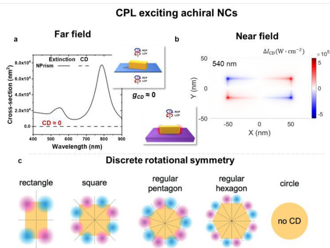
Figure 8. Local and far-field responses when CPL excites achiral plasmonic NCs. (a) Far-field signal of a Au nanoprism of 110 \times 40 \times 40 \text{ nm}^3 . The plot shows the computed far-field extinction profile of the structure in aqueous solution, also indicating its negligible CD. Inset: Schematic diagram of the Au nanoprism being illuminated by LCPL or RCPL, and an equal fraction of their power passing through. (b) Near-field differential field pattern of the same Au nanoprism under CPL with \lambda = 540 \text{ nm} . Inset: Schematic diagram of the Au nanoprism being illuminated by LCPL or RCPL, and generating a local near-field response. (c) Schematic diagrams of local patterns of differential near-field excitation arising when achiral NCs with increasing rotational symmetry are placed under LCPL or RCPL. The different colours indicate opposite signs of \Delta I_{CD} . Panels a and b were adapted from Ref. 180. Panel c was adapted from Ref. 79.
