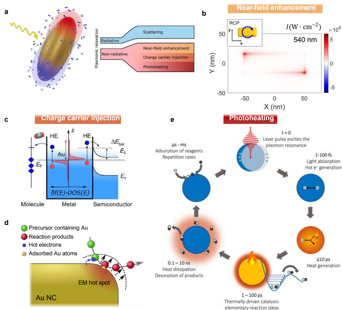
Figure 9. Energy transfer mechanisms in plasmonic photocatalysis, in the context of light-to-matter chirality transfer. (a) Schematic diagram illustrating an excited plasmonic nanostructure and its local environment. The chart indicates the main categories of mechanisms leading to the transfer of energy from the plasmonic mode into the environment. The three non-radiative processes can deposit energy locally. (b) Cross-sectional map showing the enhancement light intensity around a rectangular prism illuminated with CPL. (c) Schematic diagram depicting intraband hot electron excitation and injection from the plasmonic metal to its environment. The electrons need sufficient energy to traverse an interfacial potential barrier or reach empty molecular orbitals. A similar diagram could be shown for hole injection. A typical energy distribution of excited carriers in a plasmonic NC (red curve) is overlaid over the states of the metal. The high-energy electrons and holes excited through intraband (depicted) and interband (not depicted) transitions can induce redox reactions at the metal's surface. (d) Diagram depicting the general mechanism of ion aggregation, one of other possible redox reactions that can lead to NC growth. (e) Schematic diagram of the steps involved in a photocatalyst prepared to drive a reaction thermally, under pulsed illumination. Panel b was adapted from Ref. 180. Panels c and d were adapted from Ref. 55. Panel d was adapted from Ref. 214.
