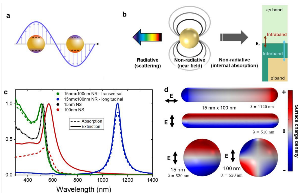
Figure 6. (a) Schematic diagram of a plasmonic nanosphere being excited by an external electric field at a frequency lower than its resonance frequency. The charges follow the external field excitation and accumulate on the metal surface. (b) All the different decay processes involved in a nanoparticle after interacting with an electromagnetic field. (c) Normalized absorption and extinction cross section for different-sized nanoparticles (diameters of 15 nm and 100 nm) and a 15 nm x 100 nm nanorod (longitudinal and transversal mode). (d) The surface charge density for a 15 nm nanosphere and a 15 nm x 100 nm nanorod at their corresponding plasmon resonance.
