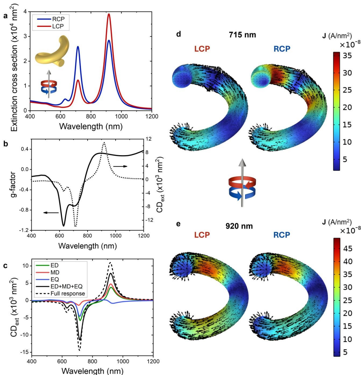
Figure 7. (a) Extinction cross section of a gold chiral helix (inset). (b) Extinction g -factor (left axis), circular dichroism (right axis). (c) Comparison of CD from the extinction obtained from the full field simulation and from the multipolar expansion of the dynamic charge distribution up to the electric quadrupolar moment. The figure also includes the curves arising only from the electric dipole (ED), magnetic dipole (MD), and electric quadrupole (EQ). (d,e) Current density, alongside normalized vector fields showing their direction, when excited at a wavelength of 715 nm and 920 nm for RCP and LCP. Insets in panels a and d,e show a grey arrow marking the direction of propagation of the incident light, and red and blue circular arrows indicating the direction of rotation for the electric field of LCPL and RCPL, respectively. Data in all the panels were obtained under this single illumination condition. The helix has a radius of 30.5 nm and a pitch of 70 nm, while the wire has a radius of 10.5 nm. We arbitrarily chose a right-handed helix; a left-handed helix would show opposite results.
