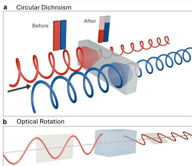
Figure 3. (a) Schematic diagram of the phenomenon of circular dichroism, showing the differing attenuation for RCP and LCP light rays traveling through a chiral medium. This differential absorption is also depicted through bars indicating the amplitude of the different CPL beams before and after they cross the material. (b) Schematic diagram of the phenomenon of optical rotation, showing how a linearly polarized plane wave has its polarization plane rotated along the direction of propagation when travelling through a chiral substance.
