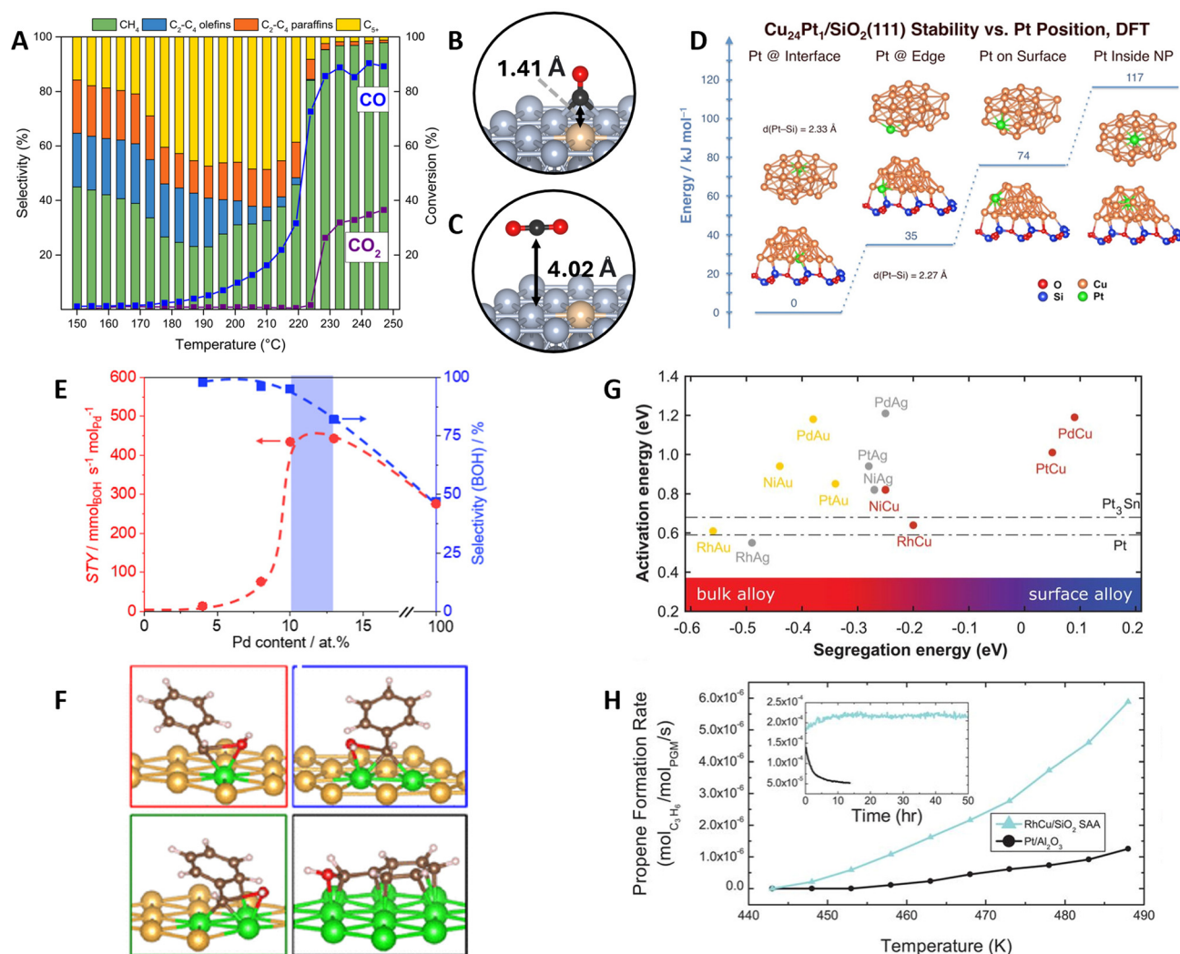
Fig. 7 DA applications in heterogeneous thermal catalysis. (A) Programmed temperature reactor studies on the reactive separation of CO/CO 2 mixtures over RuCo SAA (reaction conditions: P = 300 \text{ psig} , \text{H}_2:\text{CO}_x ratio = 2.5 : 1, \text{CO}_x = 50\% \text{ CO}/50\% \text{ CO}_2 , \text{GHSV} = 84\,000 \text{ mL h}^{-1} \text{ g}^{-1} , T = 150\text{--}250 \text{ }^\circ\text{C} , 10 \text{ }^\circ\text{C h}^{-1} ). Side views and vertical distances for (B) CO and (C) \text{CO}_2 adsorption on the RuCo SAA surface, reproduced with permission from ref. 107. (D) DFT-calculated formation energies of \text{Cu}_{24}\text{Pt}_1 nanoclusters supported on \text{SiO}_2(111) showing the stabilization of the Pt promoter on the inner SAA-support interface, reproduced with permission from ref. 120. (E) Space-time yield (STY) and BOH selectivity as a function of Pd content on PdAu DAs (reaction conditions: T = 323 \text{ K} , P = 5 \text{ bar} , F(\text{H}_2) = 50 \text{ mL STP per min} , F(\text{BA}) = 0.05 \text{ mL min}^{-1} , W_{\text{cat}} = 40 \text{ mg} ) and (F) changes in PhCHOH* C–O cleavage transition state over PdAu(111) DAs (Pd monomer, dimer, trimer) and Pd(111), reproduced with permission from ref. 125, copyright 2023 American Chemical Society. (G) Computational screening of SAA catalysts for nonoxidative propane dehydrogenation using the E_{\text{act}} of the first C–H cleavage of \text{CH}_4 and the E_{\text{seg}} as design parameters. Dash-dotted lines correspond to the E_{\text{act}} on Pt(111) and Pt 3 Sn(111) ( 2 \times 2 ). (H) Reactor studies comparing the selected RhCu/SiO 2 SAA catalyst with Pt/Al 2 O 3 (reaction conditions: 1.4 kPa of propane and 0.7 kPa of hydrogen; 90 mL min -1 flow rate. Formation rate was normalized per mole of Pt-group metal). The figure inset corresponds to the stability test performed for 50 h at T = 623 \text{ K} , reproduced from ref. 101 with permission of the American Association for the Advancement of Science.
