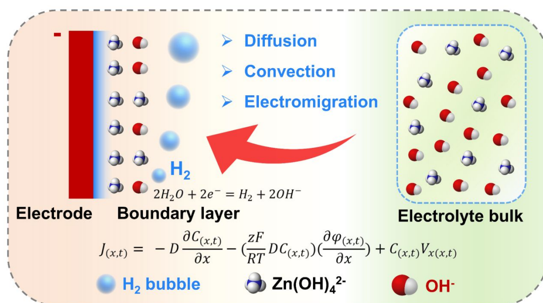
Figure 1. Diffusion, electro-migration, and convection of zincate (take alkaline media
