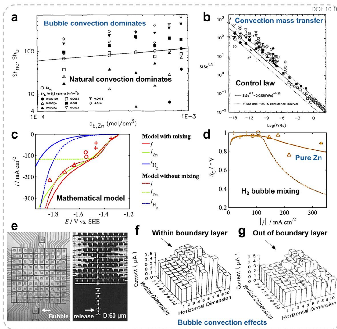
Fig. 6 (a) Sherwood number comparison: natural vs. bubble convection. (b) Dimensionless correlation comparison of various systems. Reproduced from ref. 40 with permission from IOP Science, copyright 1992. Experimental and simulated (c) polarization curves and (d) current efficiencies of Zn electrode, with Zn deposit morphologies, at 0.767 M. Reproduced from ref. 42 with permission from Elsevier, copyright 2017. (e) Micromosaic electrode (left) and hydrogen bubbles rising along it (right). (f) Spatial distribution of mass-transfer rate enhanced by 60 \mu\text{m} hydrogen bubbles generated by 8.5 \mu\text{A} current rising within the mass transfer boundary layer. (g) Spatial distribution of mass-transfer rate enhanced by 100 \mu\text{m} hydrogen bubbles
