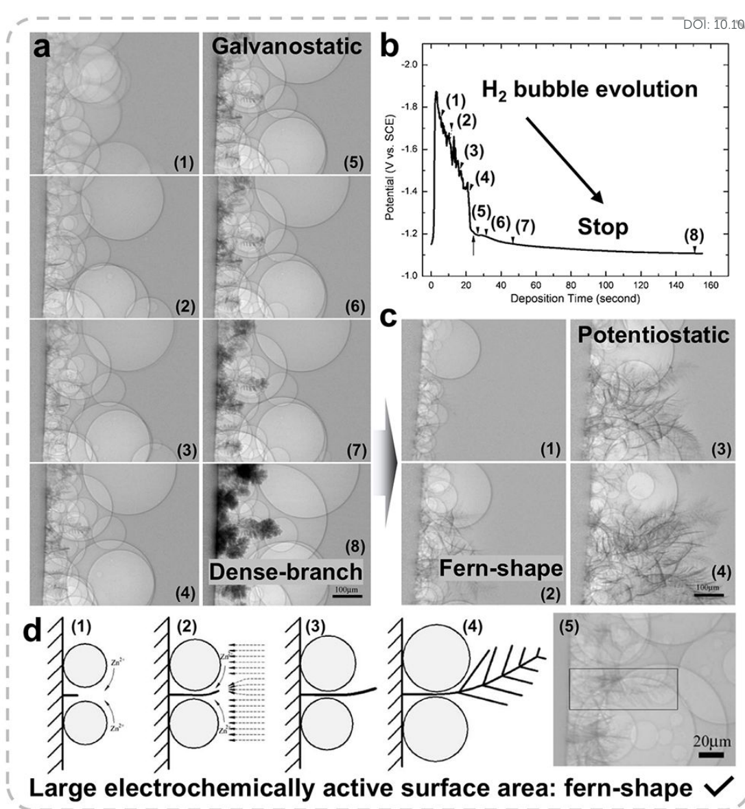
Fig. 10 (a) Microradiographs of Zn deposition on a copper substrate (on the left) with galvanostatic plating at the current density of 200 \text{ mA cm}^{-2} . The images correspond to the times of (1) 5.4, (2) 10.6, (3) 15.8, (4) 21, (5) 26.2, (6) 31.4, (7) 47, and (8) 151 s. (b) Potential transient curve at the current density of 200 \text{ mA cm}^{-2} . The arrow labeled 1-8 corresponds to the microradiographs in (a). (c) Microradiographs of fern-shaped dendrites growth at -1.8 \text{ V} at times of (1) 5.4, (2) 10.6, (3) 15.8, and (4) 21 s. (d) Schematic of fern-shaped dendrite formation with hydrogen bubbles and electric field.
