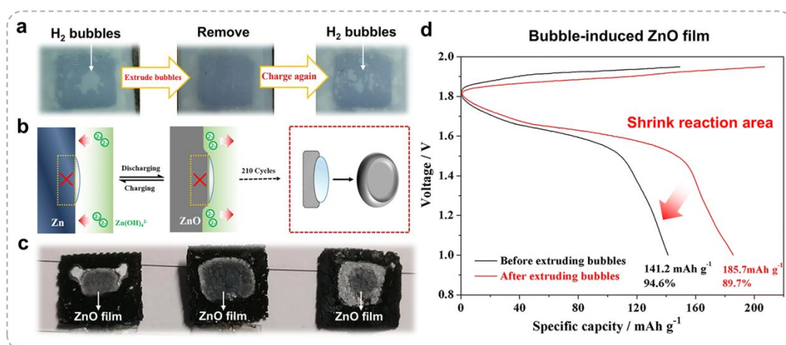
Fig. 5 (a) Hydrogen bubble formation on Zn electrode back. (b) Schematic diagram of the hydrogen bubble effect on Zn electrode deformation. (c) Zn anode after 210 cycles. (d) Electrochemical performance before/after bubble extrusion. Reproduced from ref. 37 with permission from Springer, copyright 2021.
