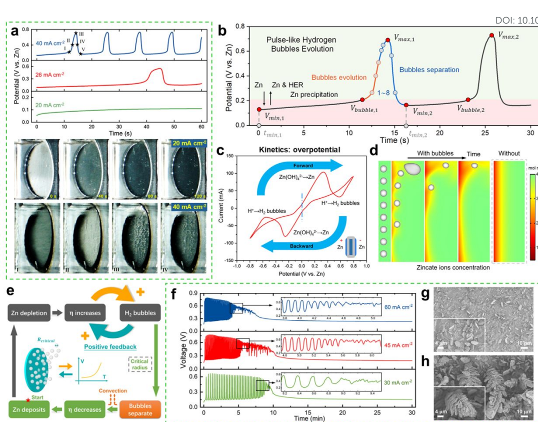
Fig. 2 (a) Potential profiles during Zn deposition at current densities of 20, 26, and 40 mA cm -2 , along with electrode images at 20 and 40 mA cm -2 . (b) Potential oscillations with characteristic parameters. (c) CV curve of symmetric Zn electrodes. (d) Zincate ion concentration distribution with and without bubble separation. (e) Schematic of the potential oscillation mechanism. (f) Potential evolution at 30, 45, and 60 mA cm -2 over 30 minutes. (g and h) The SEM images of oscillatory and steady-state morphologies corresponding to the condition of the zinc electrode surface at the initial irregular stage and the end stable regular stage (Fig. 2f) within a current density of 45 mA cm -2 , respectively. Reproduced from ref. 35 with permission from Elsevier, copyright 2022.
