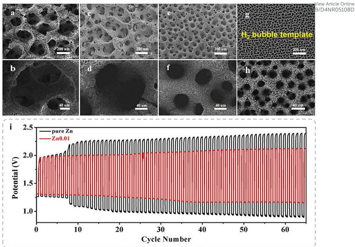
Fig. 11 Electrodeposited 3D porous Zn structures at various Zn ion concentrations: (a, b) 0.2 M, (c, d) 0.1 M, (e, f) 0.05 M, (g, h) 0.01 M. NaBr and C_2H_3O_2NH_4 were 3 M and 1 M, respectively. (i) Zn-air battery cycling performance tests with a Zn electrode deposited with 0.01 M Zn ion and a pure Zn foil: discharge-charge tests at the current density of 5 \text{ mA cm}^{-2} . Reproduced from ref. 50 with permission from Frontiers, copyright 2019.
