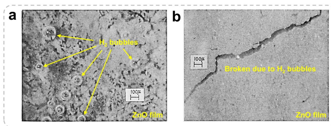
Fig. 9 (a) Hydrogen bubble emergence from ZnO film. (b) Crack in ZnO film due to hydrogen bubbles. Reproduced from ref. 47 with permission from IOP Science, copyright 1971.
