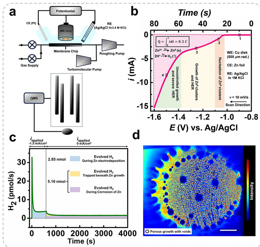
Fig. 7 (a) ECMS setup schematic, with WE, RE, and CE representing the working, reference, and counter electrodes, respectively, and QMS denoting Quadrupole Mass Spectrometer. (b) Linear sweep voltammogram for Zn deposition on Cu electrode in 0.5 M ZnSO 4 . (c) Hydrogen evolution vs. time at the current density of 1.5 mA cm -2 , current application (0-600 s) and after it stops (600-4000 s). (d) X-ray tomography image of Zn deposited at -1.5 mA cm -2 for 10 min, showing void-containing deposits (scale bar: 3 mm). The color bar indicates Zn intensity, with red signifying the highest and blue the lowest concentration. Reproduced from ref. 43 with permission from Wiley,
