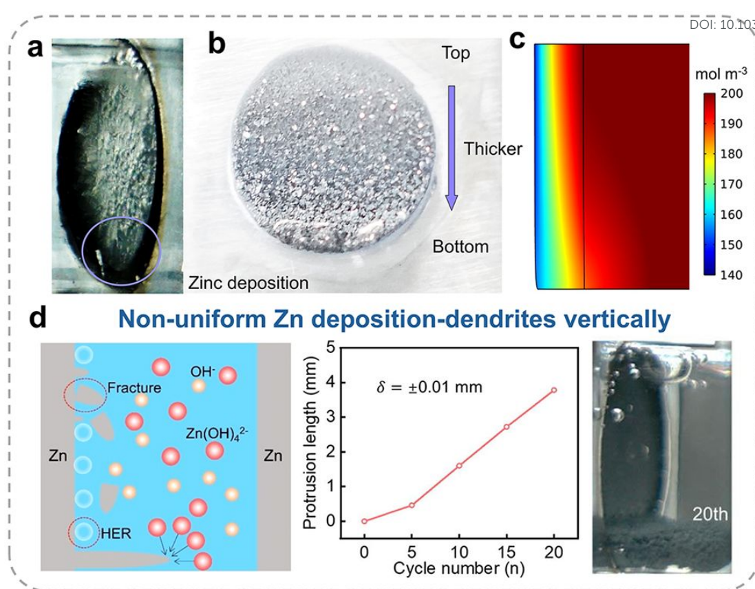
Fig. 3 (a) Zn electrode surface during initial bubble separation, with active surface concentrated at the bottom. (b) Zn electrode morphology after deposition, thicker from top to bottom. 35 Copyright (2022 and Elsevier). (c) Zincate ion distribution after 10-min deposition with hydrogen bubbles. (d) Schematical demonstration of the HER impact on Zn deposition behavior, Zn electrode protrusion length during cycles, and Zn electrode image at the 20th cycle in a symmetric Zn battery at a current density of 10 mA cm -2 . Reproduced from ref. 36 with permission from Elsevier, copyright 2022.
